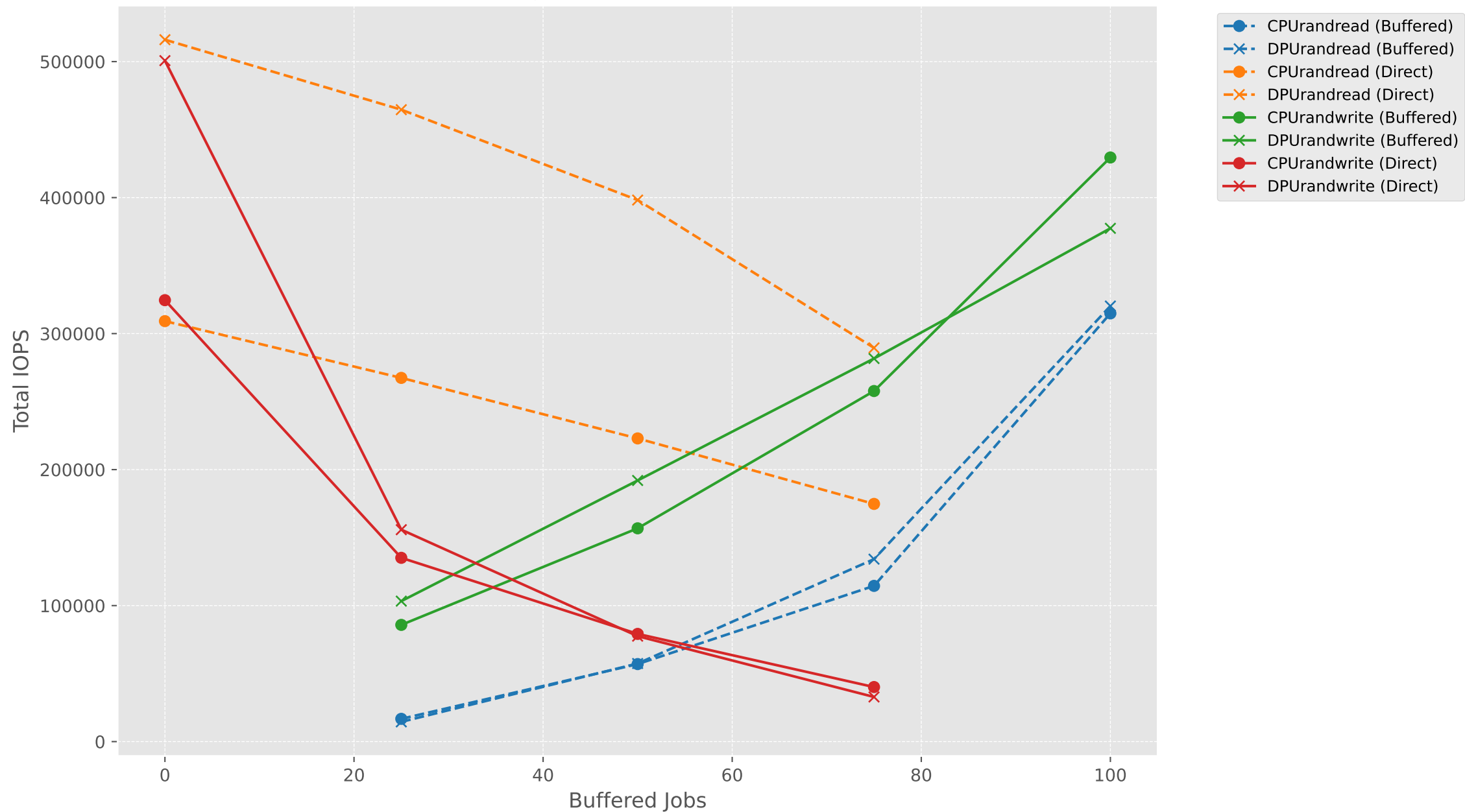
IOPS vs Buffered Jobs (mixed) - RAND (CPU vs DPU)
